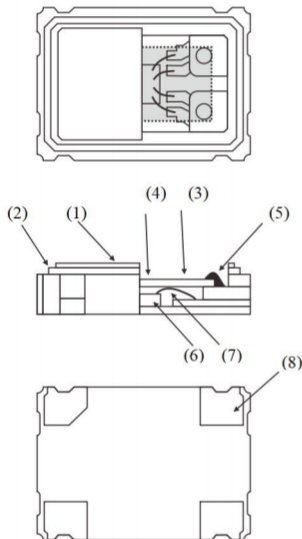
Figure 6 Internal Structure
