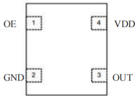
Figure 3 Pin Assignments
